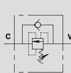
SCHEMA IDRAULICO HYDRAULIC DIAGRAM
